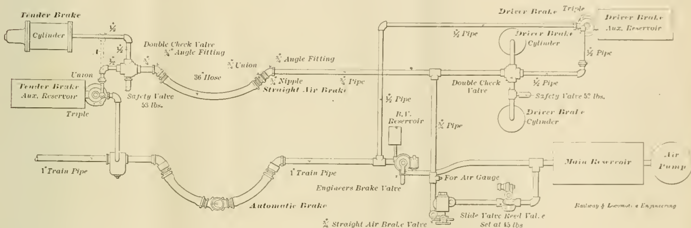
COMBINED AUTOMATIC AND STRAIGHT AIR-BRAKE.
